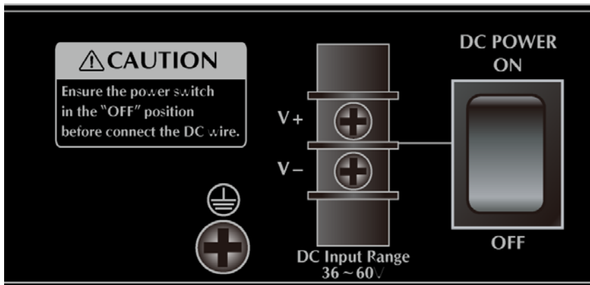
Figure 2-1-16 Rear Panel of GS-5220-16S8CR
