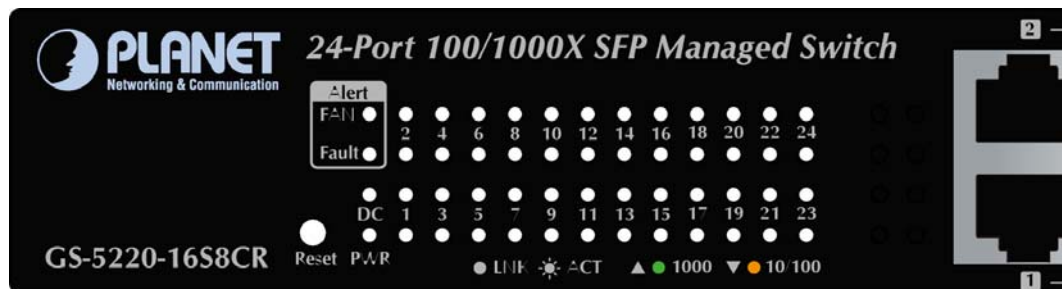
Figure 2-1-7: GS-5220-16S8CR LED on Front Panel
