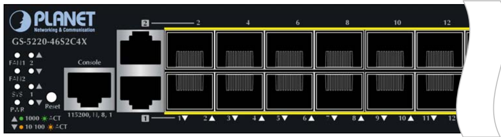
Figure 2-1-9: Front Panel LEDs of GS-5220-46S2C4X
